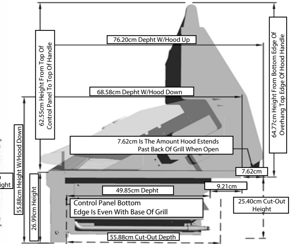
Hood Open - Right Side View
