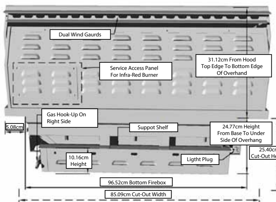
Hood Closed - Back View
