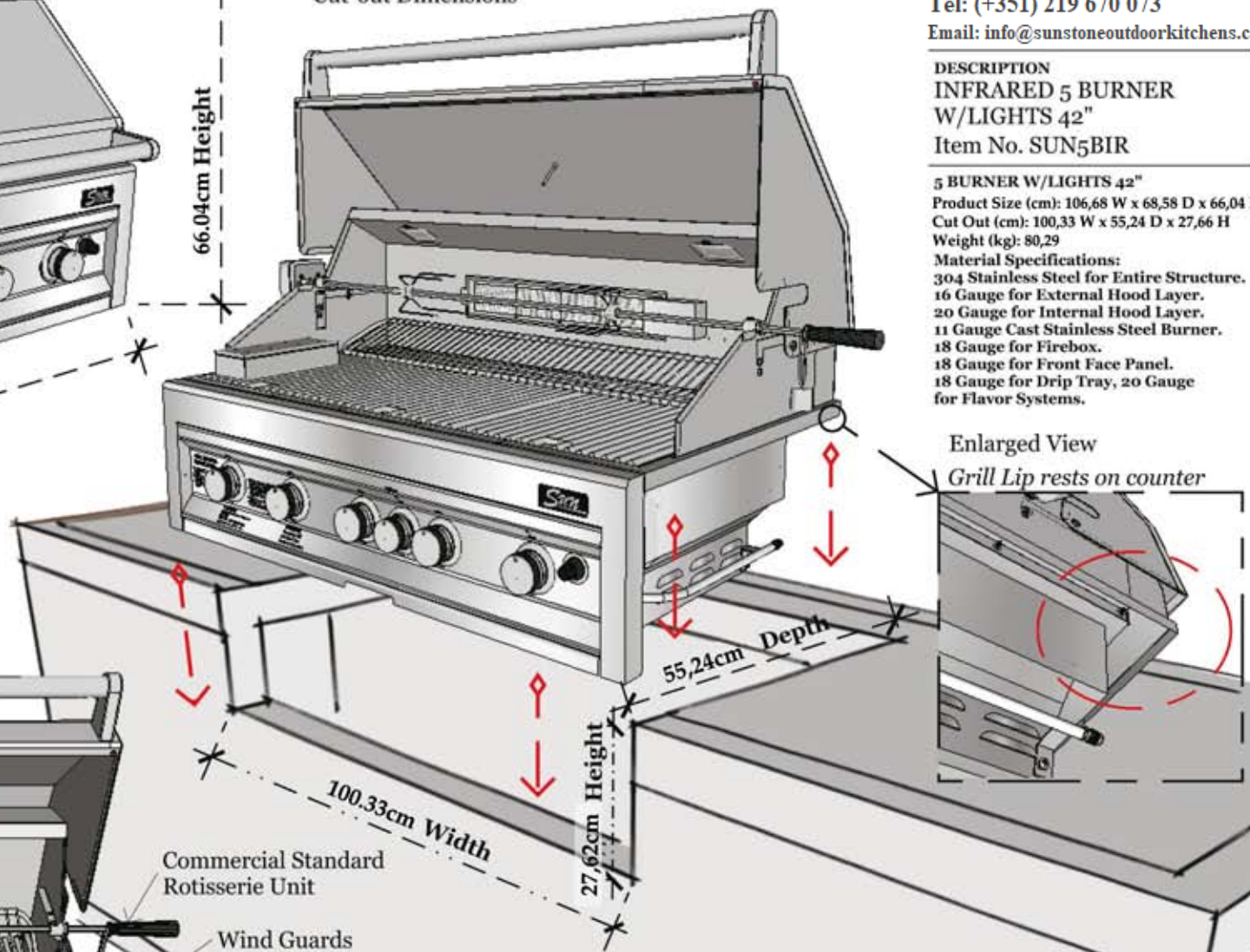
Cut-out Dimensions
